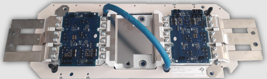
ZOPF Rotor / Line IGBT for GE 2.5 turbines
