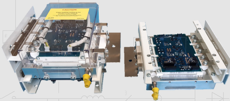
ZOPF Rotor / Line IGBT for GE 1.5 turbines
